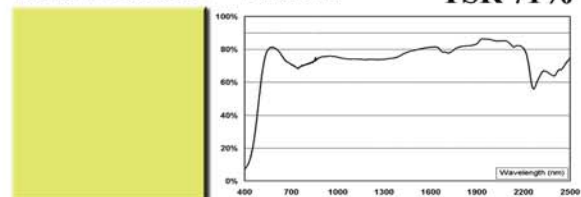
Yellow 10C112 NiSbTi TSR 71%
