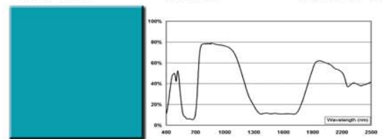
Blue 211 CoCrAl TSR 29%
